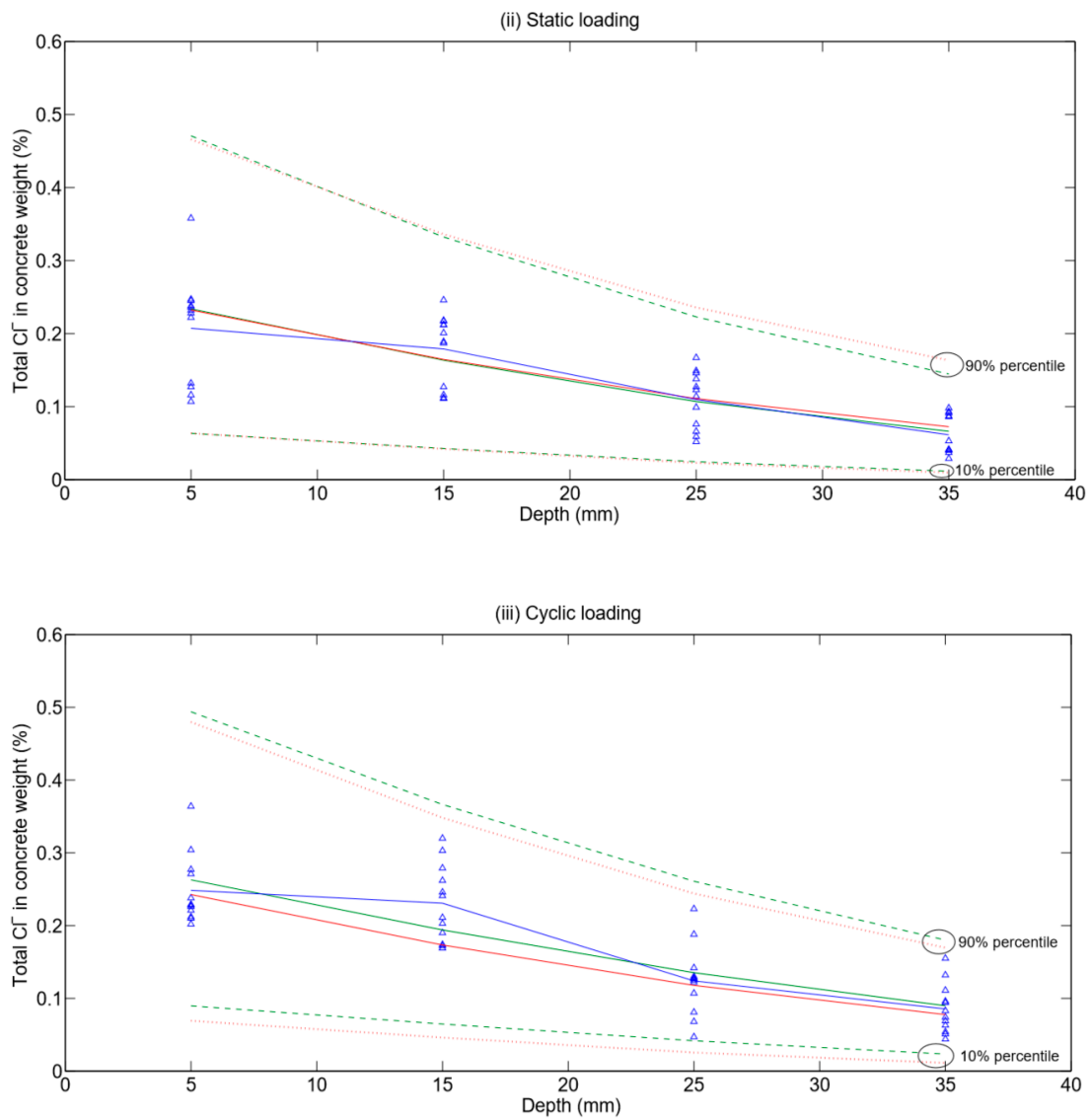
Figure 9. Comparison of chloride content into concrete at measurement depths.
