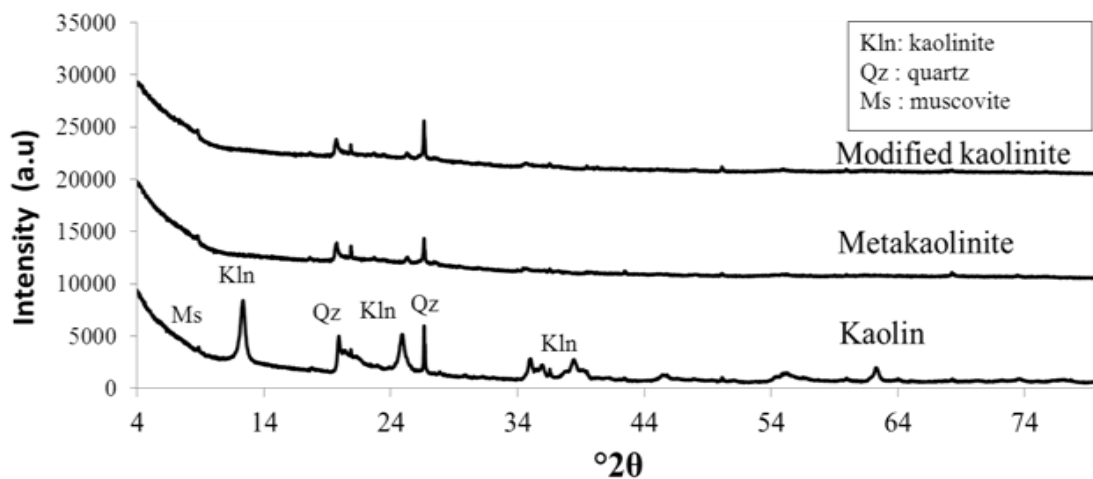
Figure 3. XRD pattern of kaolin, metakaolinite, and modified kaolinite
