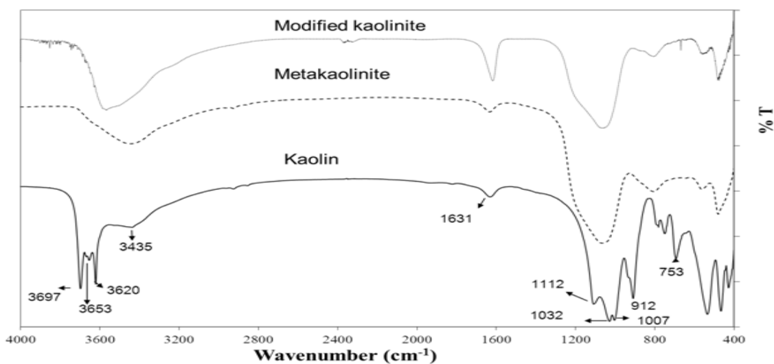
Figure 4. Infrared spectra of kaolin, metakaolinite, and modified kaolinite
