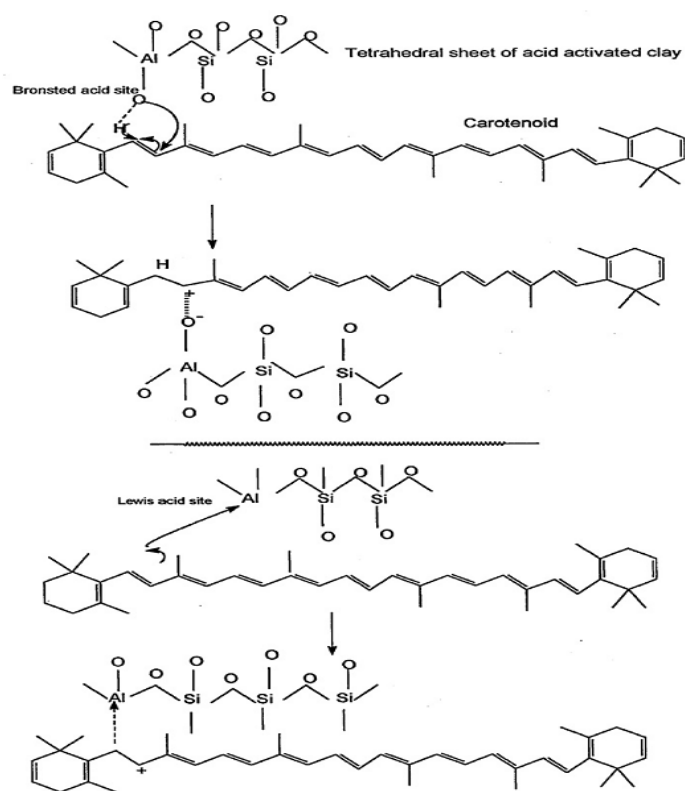
Figure 8. The mechanism of carotenoid adsorption on Brönsted and Lewis acid sites (Srasra and Trabelsi-Ayedi, 2000)
