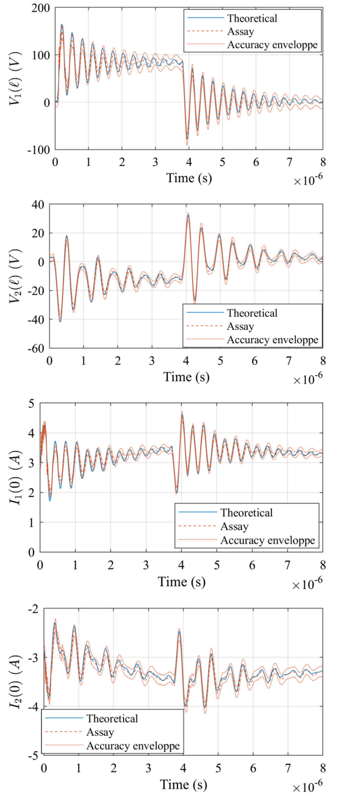
Fig. 16 Time-domain validation results
