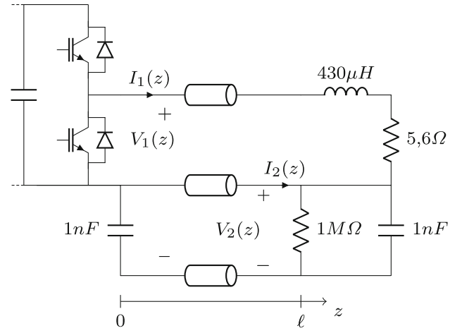
Fig. 13 Schematic for the three-conductor cable time-domain validation experiment, \ell = 12 m
