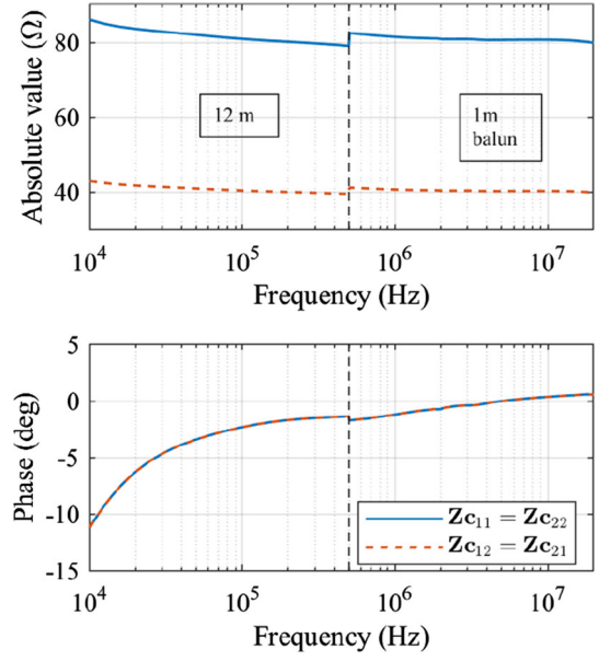
Fig. 8 Characteristic impedance
