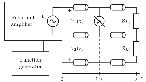
Fig. 10 Schematic of the frequency-domain validation experiment, \ell = 12 m
