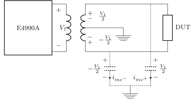
Fig. 5 Common-mode analysis of balun-isolated measurement
