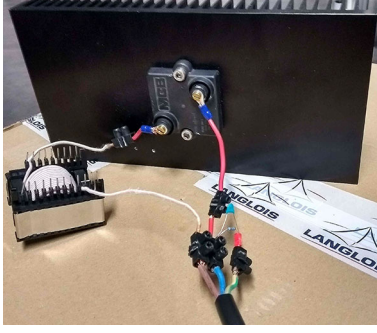
Fig. 15 Load used in the three-conductor cable time-domain validation experiment
