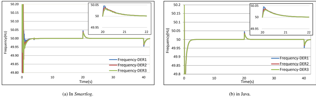
Figure 6: Frequency response after a 25 % load change and the action of both the primary and secondary controls.
