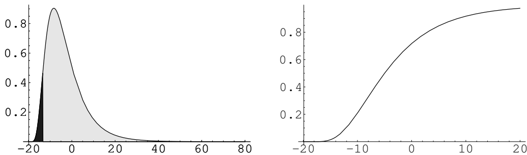
Fig. 1: Illustration of VaR for pdf and cdf
