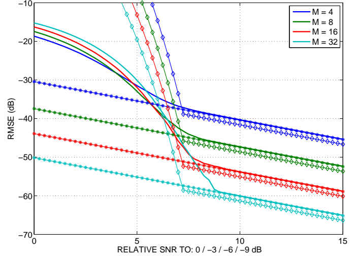
Fig. 3. MSE, CRB and WWB ( q = \frac{1}{2} ) versus SNR
