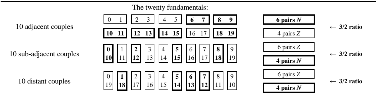
Fig. 66 Distinction of the pairs to configuration N (e-e e-m m-u u-c c-c) and to configuration Z (u-u u-e e-c c-m m-m). (See Fig. 60.) Distinction des couples de configuration N (e-e e-m m-u u-c c-c) et de configuration Z (u-u u-e e-c c-m m-m). (Voir figure 60.)
