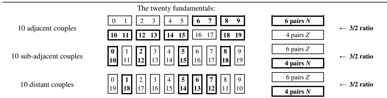
Fig. 66 Distinction of the pairs to configuration N (e-e e-m m-u u-c c-c) and to configuration Z (u-u u-e e-c c-m m-m). (See figure 60.) Distinction des couples de configuration N (e-e e-m m-u u-c c-c) et de configuration Z (u-u u-e e-c c-m m-m). (Voir figure 60.)
