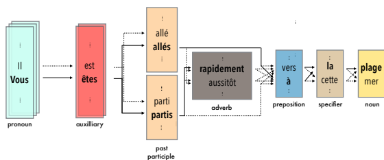
FIGURE 3 – Phrase generator functioning for the above quoted phrases, chosen words are in bold, dotted lines represent possible choices for the algorithm
