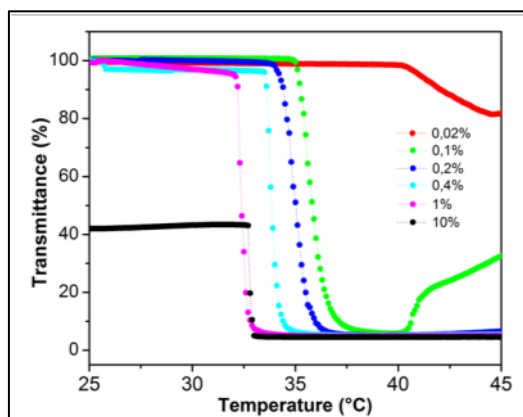
Figure 5 Effect of the concentration on the CP of aqueous solutions of P2 measured by UV-Vis (heating rate: 0.2 °C min -1 ).
