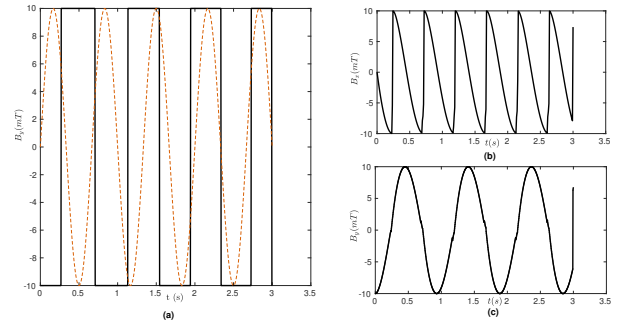
Fig. 4. Solution of the planar optimal control problems. (a) : y -component of the solution of OCP-1 compared with the sinusoidal field at optimal frequency (1.5Hz). (b) : x -component of the solution of OCP-2. (c) : y -component of the solution of OCP-3.
