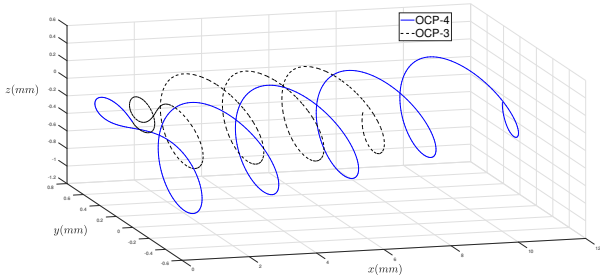
Fig. 8. Trajectories of the swimmer associated with the solutions of OCP-3 and OCP-4.
