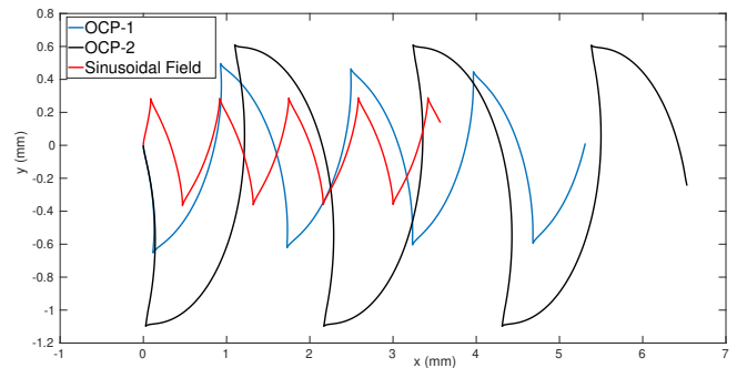
Fig. 5. Optimal planar trajectories associated with OCP-1 and OCP-2 compared with the trajectory of the swimmer actuated by the sinusoidal field.
