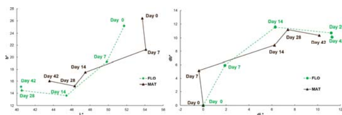
Fig. 6 Stem surface colour changes during retting measured by colorimetry (CIELab), considering the L^* (lightness) vs b^* (yellowness/blueness) components of colour (a) and relative change compared to day 0 (b).
