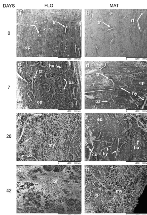
Fig. 3 SEM images of the stem surface portions of FLO (a, c, e, and g) and MAT stems (b, d, f, and h) during retting. Before retting (a,b), after 7 days (c,d), 28 days (e,f) and 42 days (g,h) of retting; (ba) bacteria, (bf) biofilm, (co) conidiophore, (ep) epidermis, (hy) hyphae, (my) mycelium, (rt) remnant of trichome, (tr) trichome and (xy) xylem. Scale bar = 300 µm.
