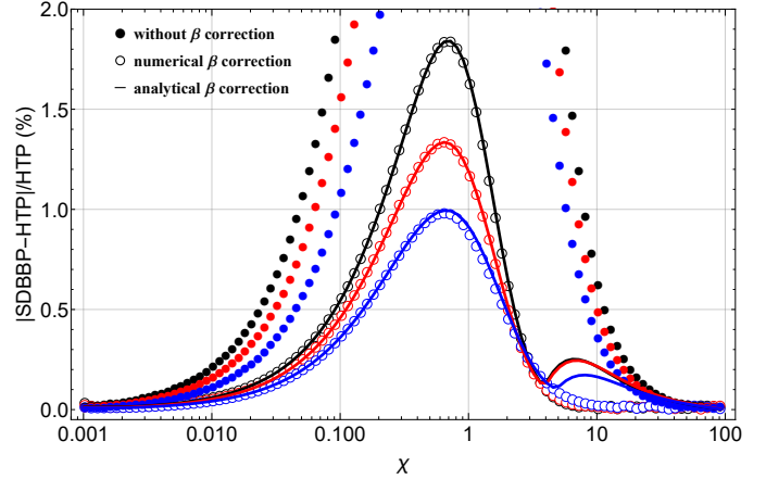
Figure 4: The relative differences between the SDBBP and the HTP simulated with the same set of parameters (note logarithmic scale of the horizontal axis). This figure partially reproduces Fig. 1. Black, red and blue colors correspond to \alpha = 0.1, 1.0 and 2.5 , respectively. Open dots represent the difference between the two profiles when numerical values of \beta are used and lines represent the same difference when analytical \beta values based on Eq. (6) are applied.
