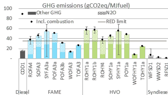
Figure 10: WtT GHG emissions of synthetic diesel compared to fossil diesel, FAME, and HVO expressed per MJ lower heating value of the obtained fuel. Combustion emissions for biofuels are assumed to equal zero. Combustion factor of fossil diesel if total combustion is supposed. Where available, error bars are added. Adapted from Edwards et al. (2013).
