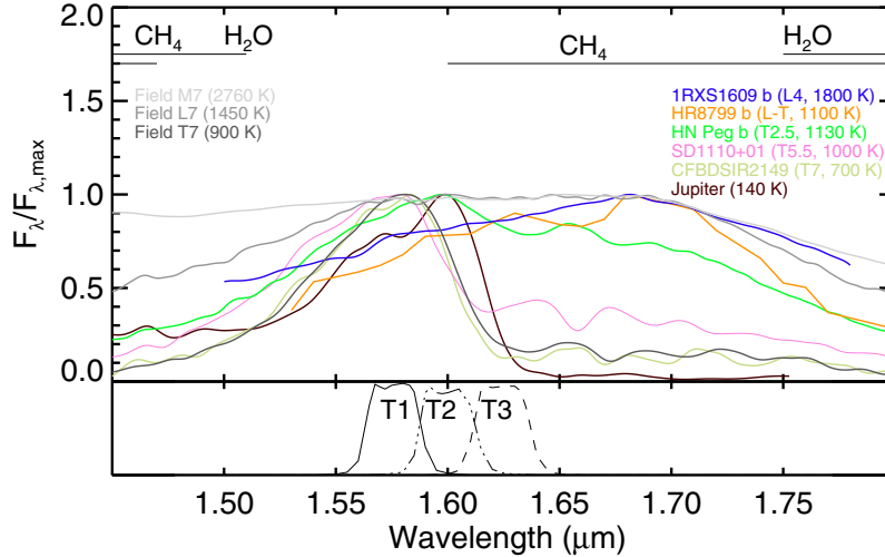
Fig. 1. Spectra at a resolution of 60 around the CH 4 band at 1.625 \mu\text{m} . Field dwarfs are from the SpeX Prism library. A peculiar red dwarf from Stephens et al. (2009) as well as young companions, free-floating planets, and Jupiter are plotted in color. They have been normalized to their highest values. The absorption bands of water and methane are labeled. The transmission of the SDI + filters (T1, T2, T3) is plotted in the bottom panel.
