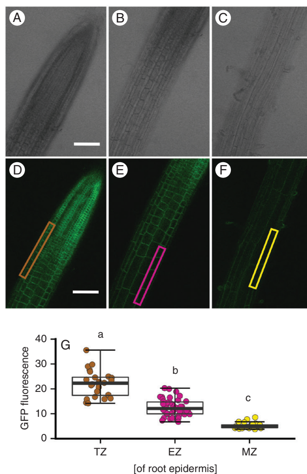
FIG. 3. DORN1 abundance declines as primary root cells mature. (A–F) Confocal microscopy images of the different zones of 14-d-old Arabidopsis root expressing a DORN1-GFP fusion from the native promoter. Epidermis in the transition zone (TZ) is marked by brown rectangle, elongation zone (EZ) by pink, and mature zone (MZ) by yellow. Scale bar = 100 µm for all. (G) Background-subtracted DORN1-GFP fluorescence of epidermis in the transition zone (TZ, brown), elongation zone (EZ, pink) and mature zone (MZ, yellow) of 14-d-old Arabidopsis roots. GFP-signal was measured from the plasma membrane of epidermal cells and normalized to cells not expressing GFP; n = 24 (TZ/MZ) and n = 44 (EZ) from six individual plants. Analysis of variance (ANOVA) with post-hoc Tukey test was used to assess statistical differences, and different letters indicate significant difference ( P < 0.001 ).
