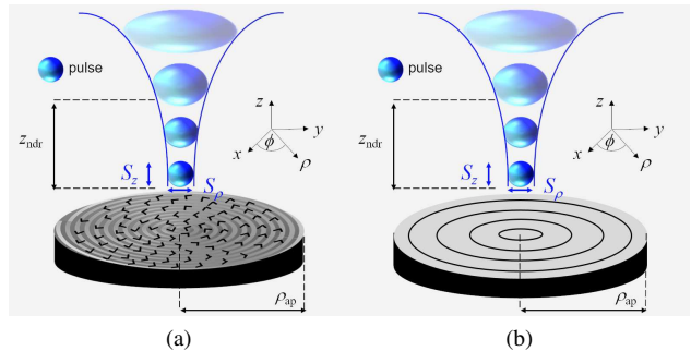
Fig. 5. (a)–(b) An X-wave is launched from (a) an RLSA antenna and (b) an LPRW. As the X-wave pulse propagates beyond the nondiffractive range z_{\text{ndr}} , the spot size increases and the intensity correspondingly decreases.
