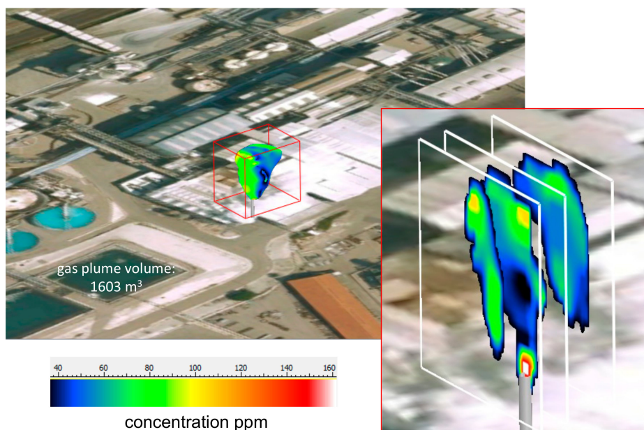
Figure 8. Experimental 3-D gOcad® modeling of the concentration of \text{NH}_3 (ppm) in the gases emitted by the chimney. The right part corresponds to a zoom of three transverse cross-sections made at three different depths in the gas cloud.
