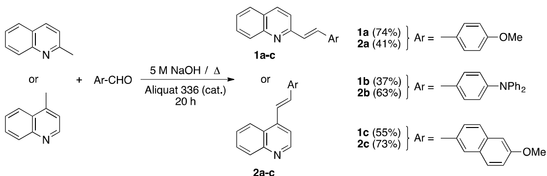
Scheme 1. Synthesis of 2- and 4-arylvinyloquinolines 1 and 2 .
