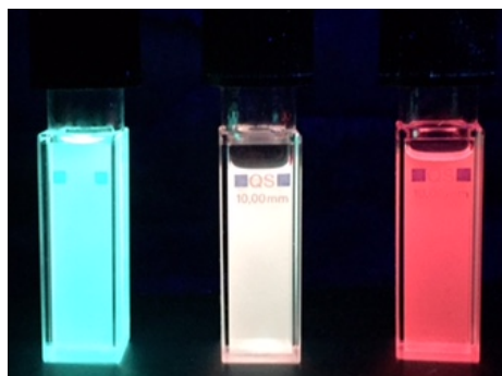
Figure 6. Changes in the color of a \text{CHCl}_3 solution of 1b ( c = 1.89 \times 10^{-5} M) after the addition of 0.9 equivalents (middle) and in 10^{-2} M CSA (right). Photographs were taken in the dark upon irradiation with a hand-held UV lamp ( \lambda_{\text{em}} = 366 nm).
