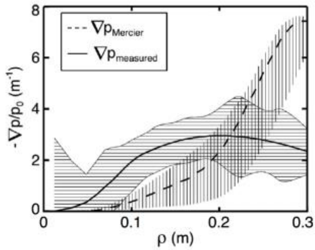
Fig. 6.1) Profile of the measured pressure gradients (solid line) in a MST discharge with pellet injection where \beta = 26\% is achieved. Dashed line is the critical Mercier pressure gradients, which is exceeded in the core plasma. Shaded regions indicate the uncertainties. From (Chapman et al., 2009)
