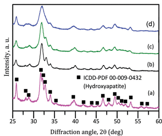
Fig. 7 Diffraction patterns of the SPS samples obtained from the amorphous powders in presence of ammonium hydroxide solution: (a) ACP; (b) cACP; (c) Mg5 cACP; (d) Mg15 cACP.
