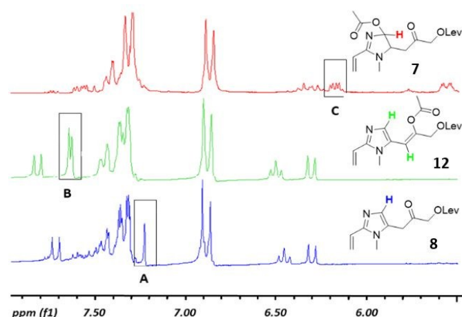
Fig. 1. Partial 1 H-NMR spectra (5-8 ppm) of acetylation products 7 (red), 8 (blue) and 12 (green). Interesting protons are highlighted (see discussion).
