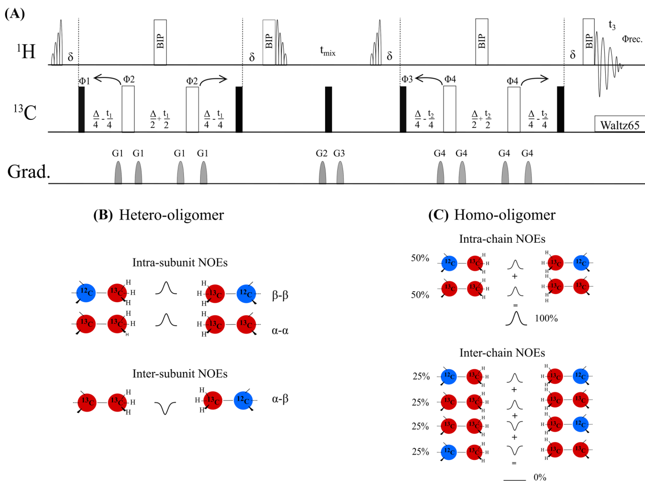
Fig. 1 Specific editing of intra vs. inter-chain methyl-methyl NOEs. a 3D CT 2 -HMQC-NOESY-HMQC pulse sequence. Excitation of proton magnetization was achieved using 1.2 ms selective 90° EBURP2 pulses covering a bandwidth of 4 ppm (Geen and Freeman 1991) and was followed by a delay \delta=4 ms for heteronuclear magnetization transfer. Methyl carbon frequencies ( F_1 and F_2 ) were encoded in constant time mode during the two multi-quantum evolution periods ( \Delta=25 ms) flanking the NOE mixing period ( t_{\text{mix}}=600 ms). 1 H chemical shift evolution during each HMQC element was refocused using a pair of high power band-selective BIP-720-50-20 1 H pulses (Kupce and Freeman 1994; Amero et al. 2009). 1.2 ms time reverse EBURB2 pulse (Lescop et al. 2010) was used to flip-back 1 H magnetization on the z-axis before the NOE mixing period. Narrow and wide bars indicate nonselective 90° and 180° 13 C pulses. 13 C decoupling during 1 H signal detection ( F_3 ) was achieved using waltz65 decoupling pulse sequence (Zhou et al. 2007). All the pulses were applied along x axis unless indicated otherwise on the figure. Phase cycling was performed as follows: \Phi_1=x, -x ; \Phi_2=x, y ; \Phi_3=x, x, -x, -x ; \Phi_4=x, x, y, y ; and receiver phase was cycled with \Phi_{\text{rec}}=x, -x, -x, x . Recycling delay was set to 1.25 s and 200 ms gradients were applied on z-axis with magnitude G_1=19 G/cm; G_2=7 G/cm;
