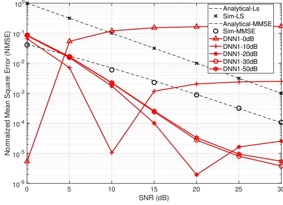
Fig. 1. NMSE Performance of DNN1 trained at different SNR values.
