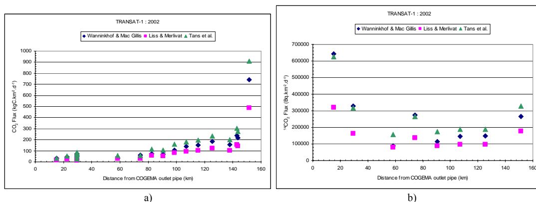
Figure 2. Variations CO 2 fluxes (a) and 14 C fluxes (b) in surface seawater versus distance from pipe outlet during TRANSAT 1.
