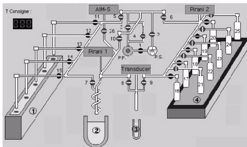
Figure 1 Schematic overview of the automated system. ①: movable furnace; ②: cold ( -78^{\circ}\text{C} ) or warm ( 70^{\circ}\text{C} ) water trap; ③: cold ( -173^{\circ}\text{C} ) or warm ( 40^{\circ}\text{C} ) calibrated finger trap; ④: cold ( -173^{\circ}\text{C} ) storage vials trap; P.P.: rotary pump; P.S.: turbo-molecular pump.
