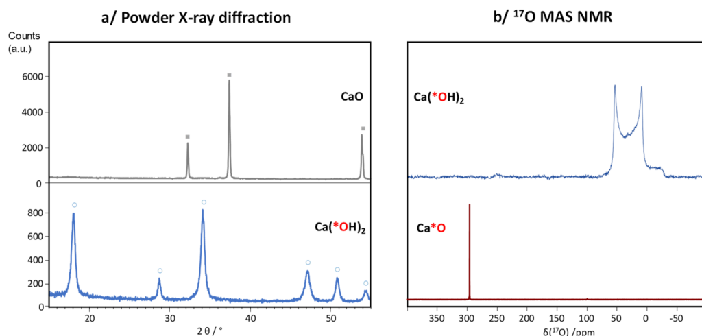
Figure 1. (a) PXRD analyses before and after LAG: CaO precursor obtained after the heat treatment of commercial Ca(OH) 2 (top) and enriched phase recovered after LAG in the presence of H 2 17 O (bottom). The symbols ■ and ○ correspond to the diffraction peaks expected for CaO (ICSD 163628) and Ca(OH) 2 (ICSD 15471), respectively. (b) Solid-state 17 O NMR spectra of 17 O-enriched Ca(*OH) 2 (prepared by LAG of CaO using H 2 17 O) and Ca*O (obtained after the heat treatment of Ca(*OH) 2 ). These 17 O MAS NMR spectra are in agreement with previous measurements at this magnetic field. 18
