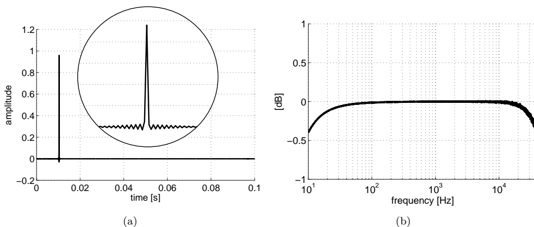
Figure 6. Estimated IR (a) and FRF (b) using the modified MLS technique (order 20). Clock frequencies of both devices are independent (asynchronous clocking mode) and are set to \approx 96 kHz as in Fig. 3.
