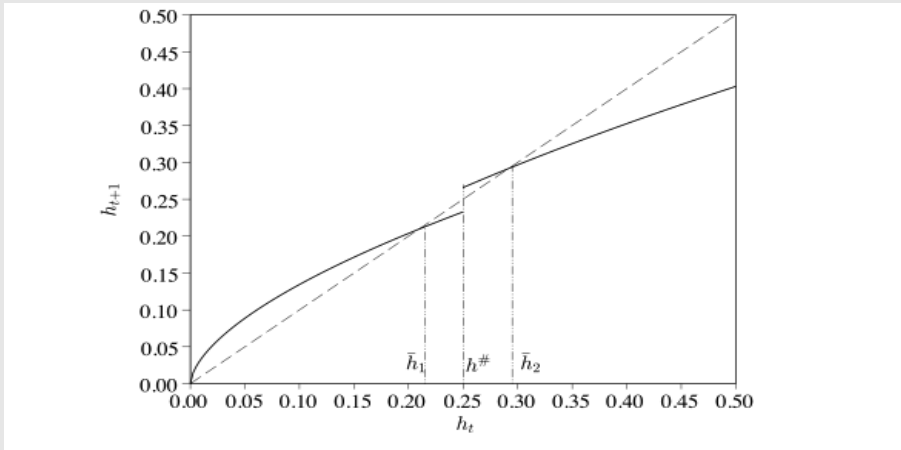
Figure 1 – The traditional case: the solid line plots recursive formula (11).
