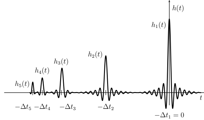
Figure 3. Result of the nonlinear convolution process y(t) * \tilde{s}(t) in the form of set of higher-order nonlinear impulse responses h_m(t) .
