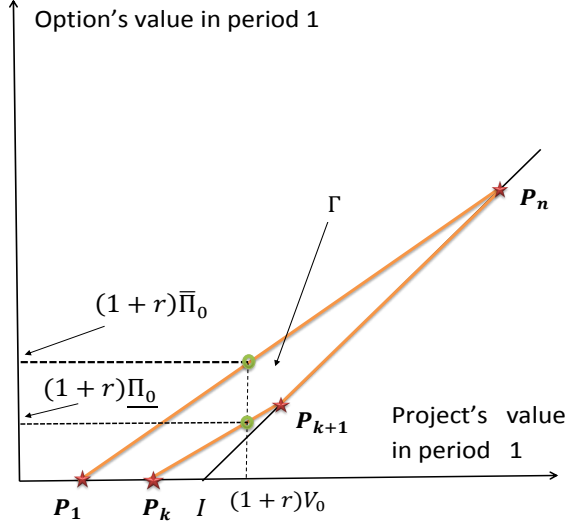
Figure 1: The convex hull \Gamma is a quadrilateral
