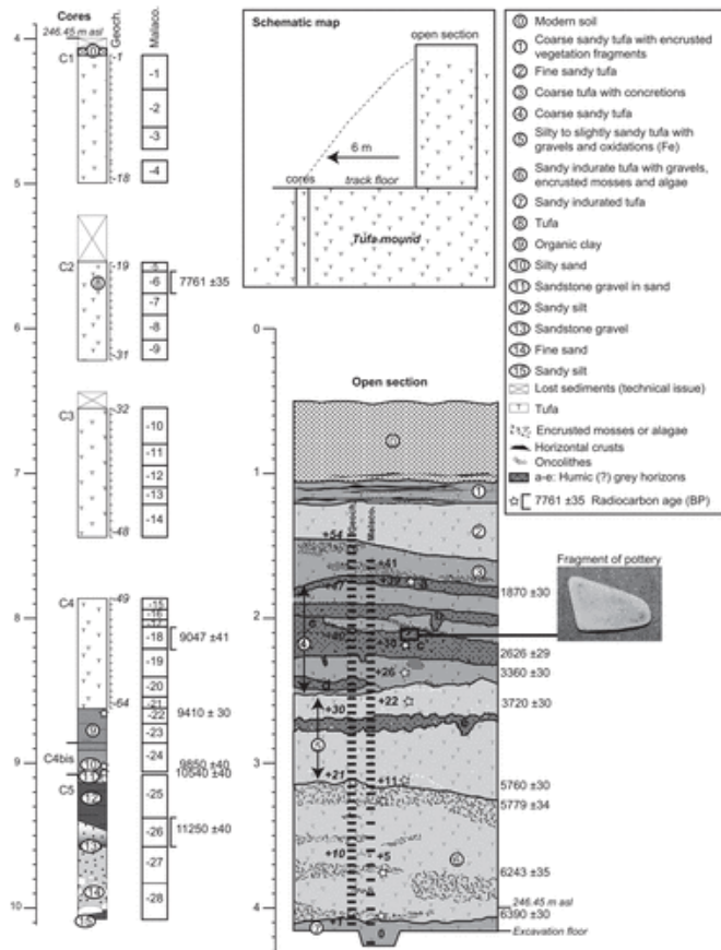
Figure 2. Schematic map of the location of the samples in the tufa mound, stratigraphy with the position of malacological and geochemical samples, radiocarbon dating and photograph of the pottery fragment found in unit 4.
