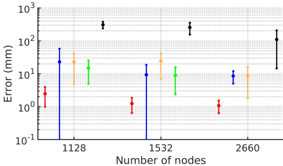
Fig. 5. Mean error and standard deviation between the needle tip and the last point of the trajectory at the end insertion for various mesh resolution.
