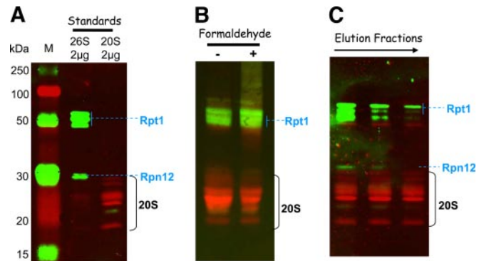
FIG. 3. Detection of 20 S core particle and 19 S activators in the purified proteasome preparations. Proteins separated by SDS-PAGE were transferred to a nitrocellulose membrane: 2 μg of commercial 20 S and 26 S proteasome from human erythrocytes as standards (A), 20 μg of total proteins from fractions containing the maximal ChT-like activity (fractions 9 and 10 from purifications without and with formaldehyde cross-linking, respectively) (B), and 10 μg of estimated 20 S proteasome (based on the ChT-like activity measurement) from fractions 8, 9, and 10 from the purification without formaldehyde cross-linking (C). Mouse monoclonal primary antibodies against 19 S proteasome subunits Rpt1 and Rpn12 and rabbit polyclonal antibodies against 20 S core subunits were used for the immunoblot staining. ECL Plex CyDye-conjugated antibodies, goat α-mouse IgG-Cy3 and goat α-rabbit IgG-Cy5, were used as secondary antibodies. The detection was performed using the Typhoon Trio fluorescence scanner at 532 nm excitation and 580 nm emission for the Cy3-conjugated antibody and 633 nm excitation and 670 nm emission for the Cy5-conjugated antibody. Lane M, molecular mass markers.
