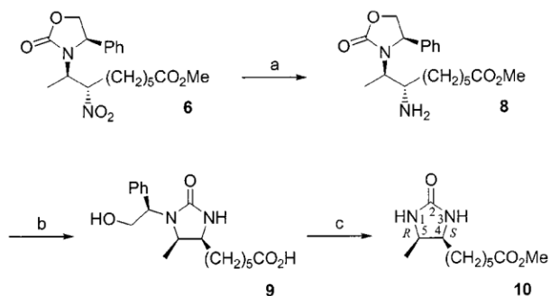
Scheme 5. Preparation of imidazolidinone 10 from nitro compound 6 ; reagents and conditions: (a) \text{HCO}_2\text{NH}_4 , Pd/C, MeOH, 3 days, 64%; (b) KOH, MeOH, 16 h, reflux, 89%; (c) \text{H}_2 , \text{Pd}(\text{OH})_2/\text{C} , MeOH, \text{H}_2\text{SO}_4 (cat.), 2 days, 64%
