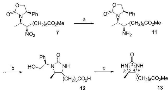
Scheme 6. Preparation of imidazolidinone 13 from nitro compound 7 ; reagents and conditions: (a) \text{HCO}_2\text{NH}_4 , Pd/C, MeOH, 3 days, 72%; (b) KOH, MeOH, 16 h, reflux, 89%; (c) \text{H}_2 , \text{Pd}(\text{OH})_2/\text{C} , MeOH, \text{H}_2\text{SO}_4 (cat.), 2 days, 63%
