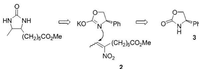
Scheme 2. Retrosynthetic analysis of dethiobiotin diastereomers
