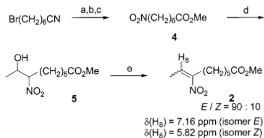
Scheme 3. Preparation of nitroalkene 2 ; reagents and conditions: (a) \text{H}_2\text{SO}_4 , MeOH, 40 h, reflux, 66%; (b) NaI, acetone, 30h, reflux, 94%; (c) \text{AgNO}_2 , ether, 3 days, room temp., 80%; (d) \text{CH}_3\text{CHO} , KOH, MeOH, 19 h, 0 °C, 84%; (e) i) DMAP, \text{Ac}_2\text{O} , ether, 16 h, room temp., ii) DMAP, basic alumina, 4 h, reflux, 63% (two steps)
