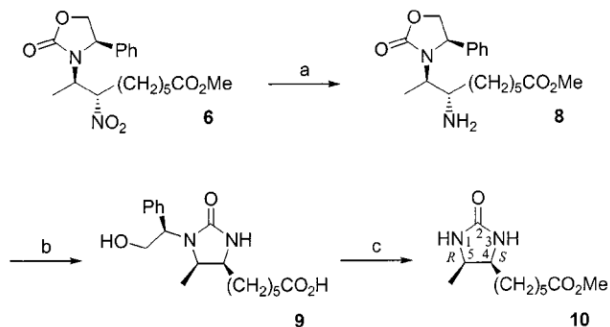
Scheme 5. Preparation of imidazolidinone 10 from nitro compound 6 ; reagents and conditions: (a) \text{HCO}_2\text{NH}_4 , Pd/C, MeOH, 3 days, 64%; (b) KOH, MeOH, 16 h, reflux, 89%; (c) \text{H}_2 , Pd(OH) _2 /C, MeOH, \text{H}_2\text{SO}_4 (cat.), 2 days, 64%
