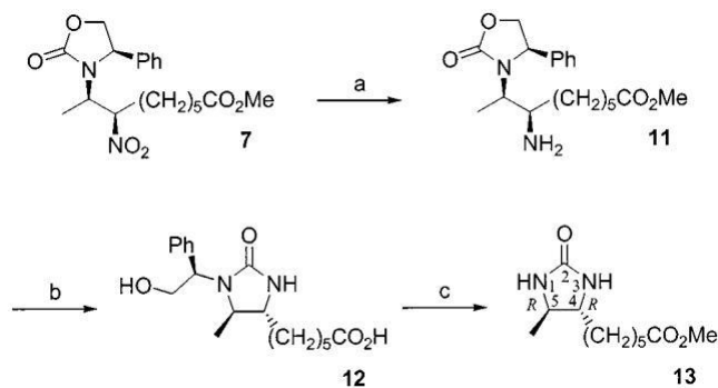
Scheme 6. Preparation of imidazolidinone 13 from nitro compound 7 ; reagents and conditions: (a) \text{HCO}_2\text{NH}_4 , Pd/C, MeOH, 3 days, 72%; (b) KOH, MeOH, 16 h, reflux, 89%; (c) \text{H}_2 , Pd(OH) _2 /C, MeOH, \text{H}_2\text{SO}_4 (cat.), 2 days, 63%
