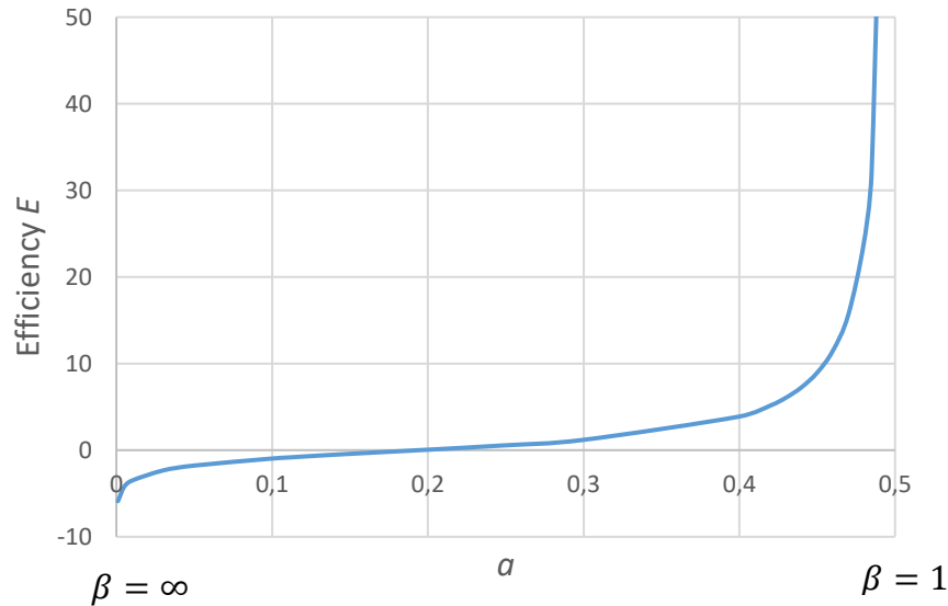
Figure 1: Evolution of the efficiency of Eq.(20) as a function of the parameter a in the interval 0 < a < 0.5 or 1 < \beta < \infty . E diverges for a=0.5 or \beta = 1 .
