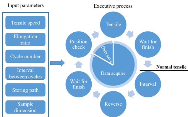
FIG. 3. Flow chart of the experiment process.
