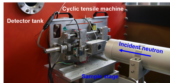
FIG. 5. The cyclic tensile machine installed on the neutron beamline of the spectrometer SANS-Suanni at CMRR.
