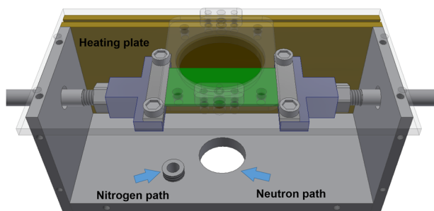
FIG. 4. Internal structure of the heating chamber. The cover and scattering window are set in transparent color for better view.
