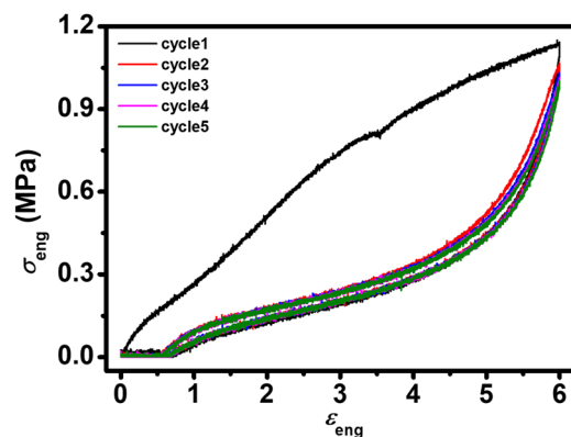
FIG. 6. Engineering stress–strain curve of MWCNT filled silicon rubber during cyclic tension. The tensile speed is 0.1 mm/s, and the initial length of the sample is 10.0 mm.
