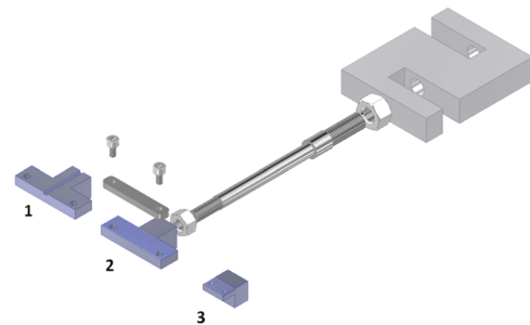
FIG. 2. Dismountable clamp for different sample parameters. 1: fiber clamps, 2: standard clamps (sample width 5–20 mm), and 3: mini clamps (sample width 1–5 mm).
