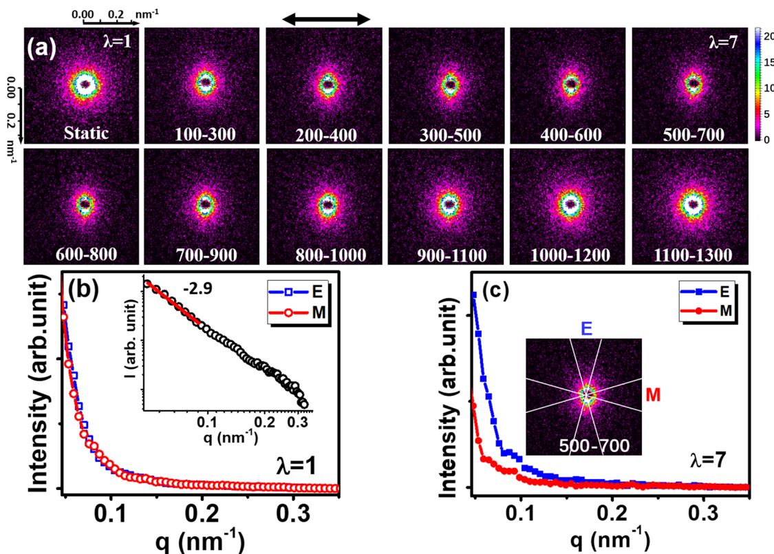
FIG. 7. (a) In situ 2D SANS patterns of the MWCNT/silicone rubber composite during the first tensile process. The numbers in the bottom of each pattern represent experimental time intervals. q_x , q_y , and z -scale are indicated in the left and right sides, respectively. The stretched direction is horizontal as indicated by the double-headed arrow. The 1D SANS profiles of the sample at an elongation ratio of \lambda = 1 and (b) and \lambda = 7 (c), respectively, in both equator (E) and meridian (M) directions. The inset 1D profiles in (b) show the power-law fitting in a log-log plot. The inset 2D SANS pattern in (c) shows the mask protocol used for integration.
