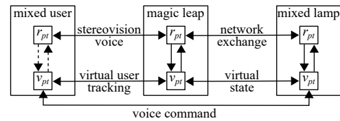
Figure 10: Adapting the MIS presented in Figure 9 to an MIS composed of a user, a Magic Leap and a mixed lamp, with vocal interactions.
