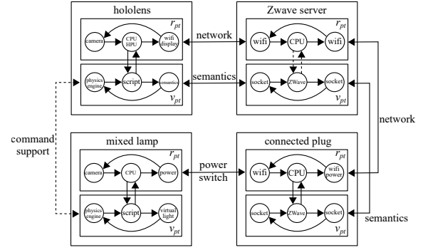
Figure 12: The internal model based on DOMIM of the use case subsystem composed of a Hololens, a ZWave server, a smart plug, and a lamp.
