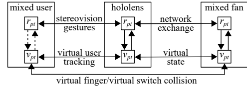
Figure 9: The external model based on DOMIM of the use case subsystem composed of a user, a Hololens and a mixed fan in the case of interaction B.
