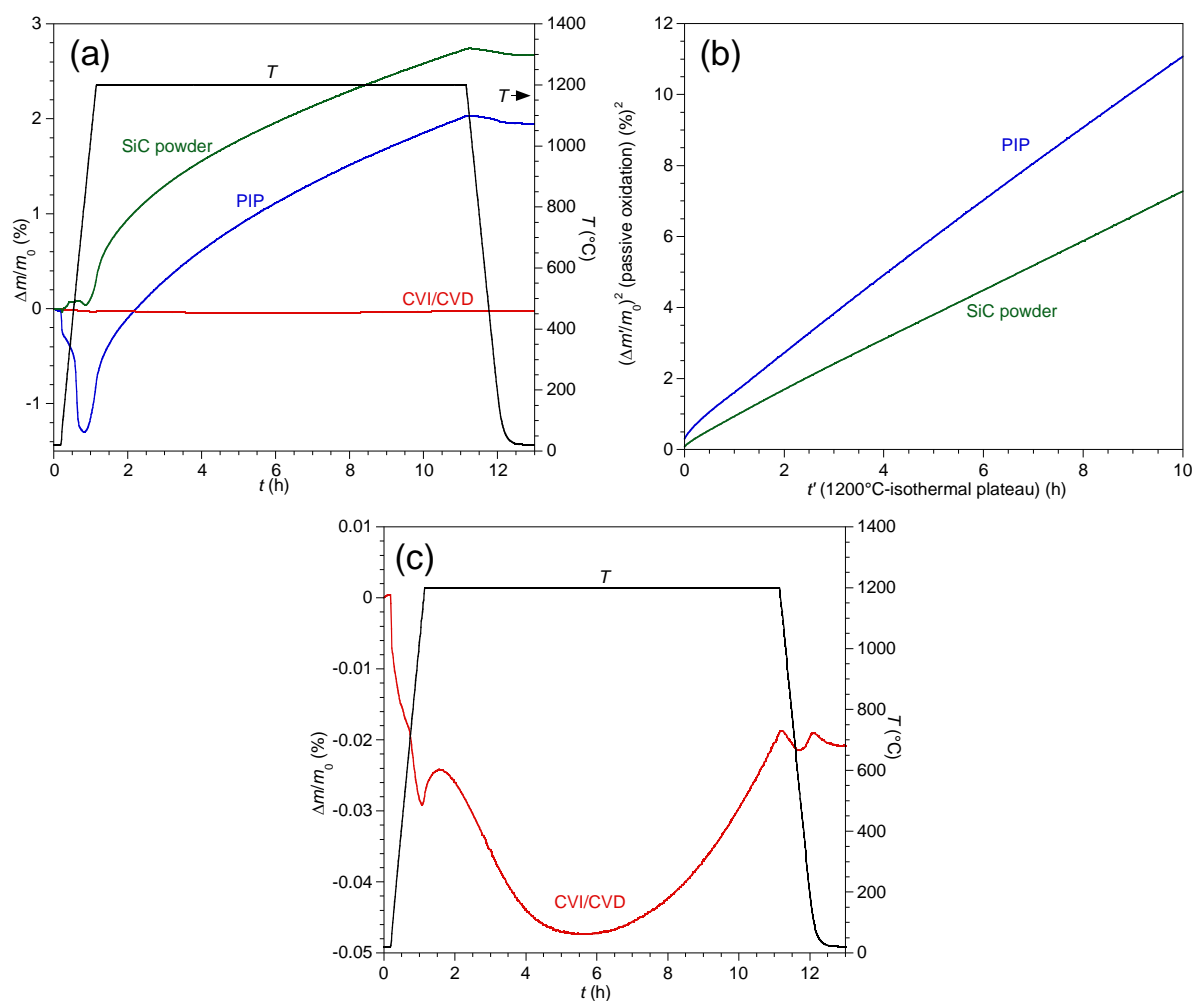
Fig. 21. (a) Relative weight change in dry air as a function of time recorded for the reference \alpha -SiC powder, the PIP lattice structure and the CVI/CVD lattice structure. (b) Square of the relative weight change as a function of time recorded for the \alpha -SiC powder and the PIP lattice structure, during the isothermal plateau at 1200 ^{\circ}\text{C} . (c) Relative weight change in dry air as a function of time recorded for the CVI/CVD lattice structure (closer view of the data presented in Fig. 21.a)
