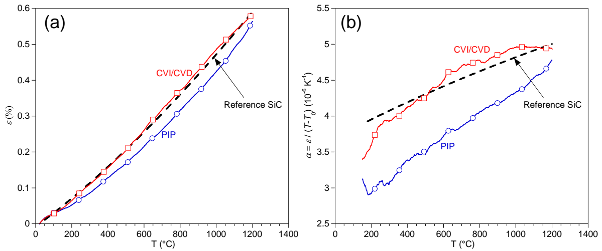
Fig. 13. (a) Thermal strain \varepsilon and (b) thermal expansion coefficient \alpha of the PIP and CVI/CVD lattice structures, as measured by thermomechanical analysis
