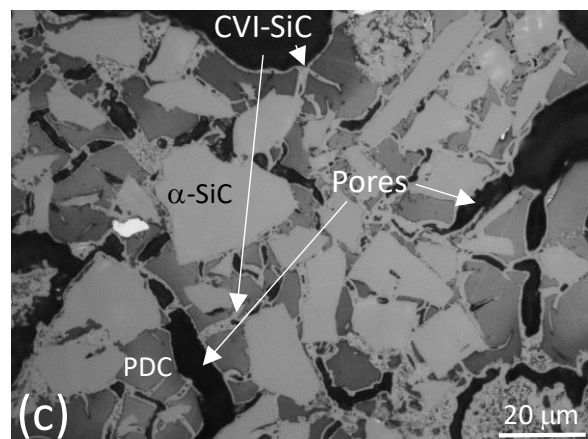
Fig. 6. Strut cross-section of a in a CVI lattice structure: (a) overview, (b) close view near the surface, (c) close view of the core
