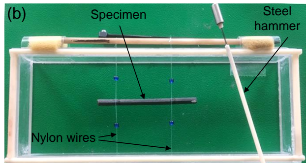
SupMat 2: (a) Schematic and (b) upper view of the testing device used for acoustic analysis
