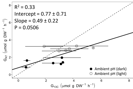
Figure 4. Calcification rates estimated based on the alkalinity anomaly technique ( G_{AT} ) as a function of calcification rates estimated based on ^{13}\text{C} incorporation technique ( G_{13C} ). The dashed line represents the 1 : 1 relationship while the full line represents the model II regression relationship. Horizontal error bars represent standard errors (SE) associated with the estimation of G_{13C} . Vertical error bars representing SE associated with the estimation of G_{AT} are too small to be visible. The corresponding dataset can be found in Table S1.
