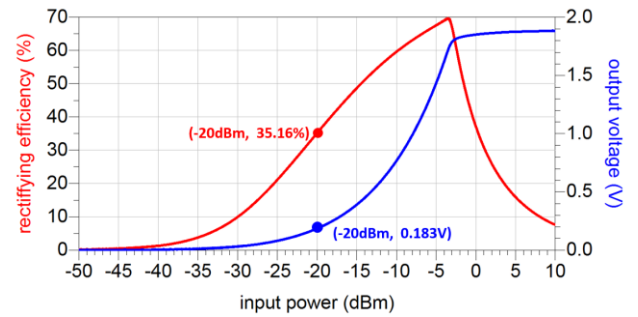
Fig.12. Topology and rectifying results for Skyworks 7630 diode (rectifying efficiency = 35.16%, output voltage = 0.183V with -20dBm input power)
