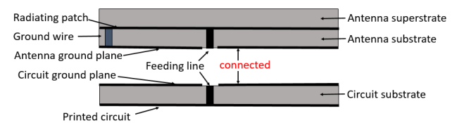
Fig.6. Rectenna system structure (physical)
