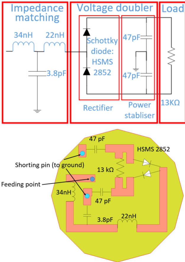
Fig.10. Three-component rectifying system design
