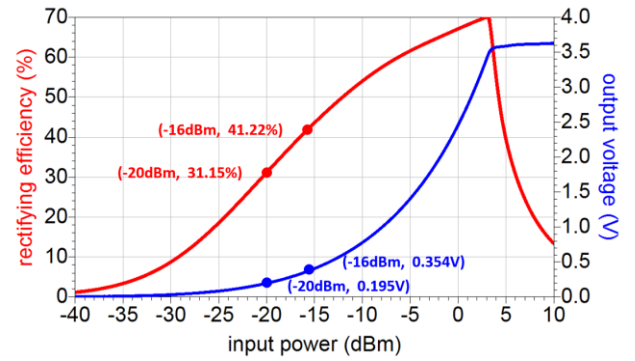
Fig.8. Efficiency and output voltage results for different input power (rectifying efficiency = 41.22%, output voltage = 0.354V with -16dBm input power; rectifying efficiency = 31.15%, output voltage = 0.195V with -20dBm input power)
