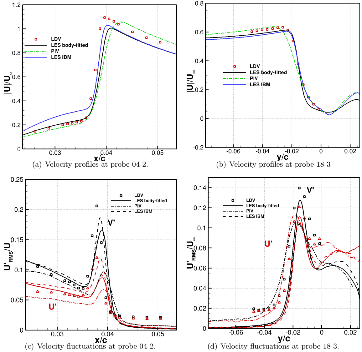
Figure 17: Comparison of velocity profiles and velocity fluctuations at probes 04-2 and 18-3. IBM simulation is compared against the reference LES simulation, PIV and LDV data.
