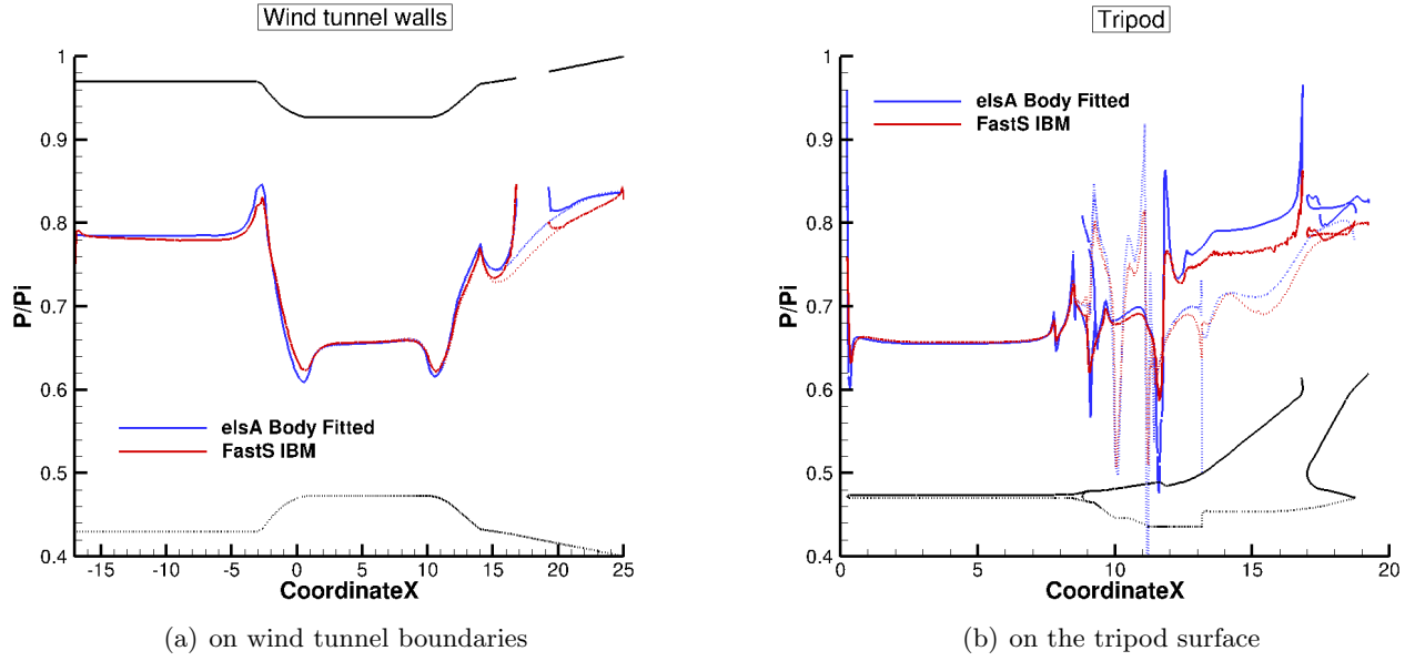
Figure 11: Comparison of the pressure along the axial direction on the wind tunnel, dashed lines denote the lower side of the tripod or of the wind tunnel. Courtesy of Aurélia Cartieri, ONERA/DS for elsA results.
