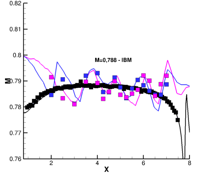
(c) Isentropic Mach number on the top curves
