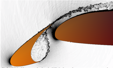
(b) Wall-modeled IBM solution near the slat.
