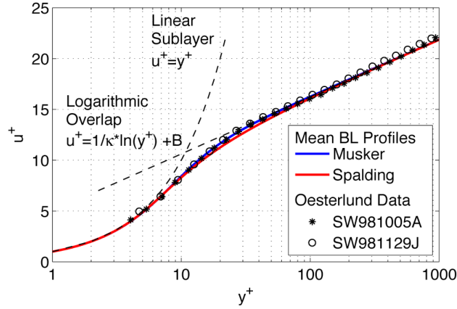
Figure 18: Asymptotic behaviors of an equilibrium boundary layer.
