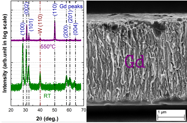
FIG. 1: The XRD results in log scale and a topographical image of Gd thick film deposited at 550°C are shown on the left and right hand side, respectively. In the XRD figure at the left hand side, the olive and purple curves are the RT and 550°C films, respectively.
