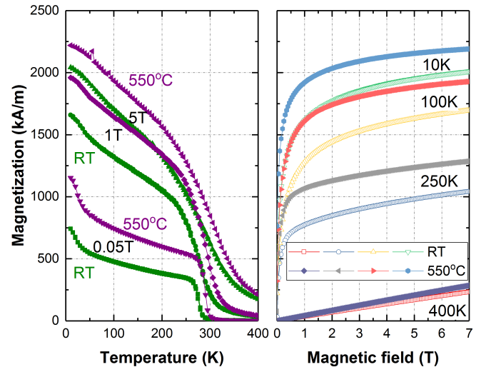
FIG. 2: M(T) curves under magnetic fields: 0.05 T, 1 T, 5 T for Gd thick films deposited at RT and at 550°C in the left hand side. The right hand side figure is a comparison of isothermal magnetization curves measured at 10K, 100K, 250K and 400 K on RT (empty symbol) and 550°C (full symbols) deposited samples.
