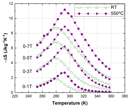
FIG. 3: Entropy change of samples deposited at RT and 550°C
