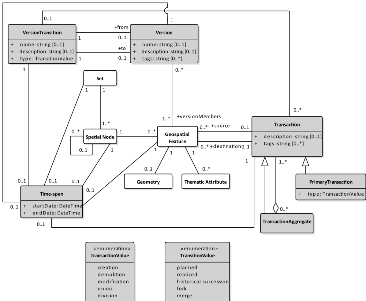
Figure 4. Gen4DCity : A generic UML conceptual model for delivering time-evolving 3D city models on the web based on 3D Tiles and I3S standards. Entities from Gen3DCity (from Figure 3) appear in white, and entities for temporal information manifest in grey.
