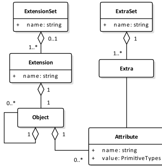
Figure 7. Description of the concepts for extending 3D Tiles as a UML conceptual model.
