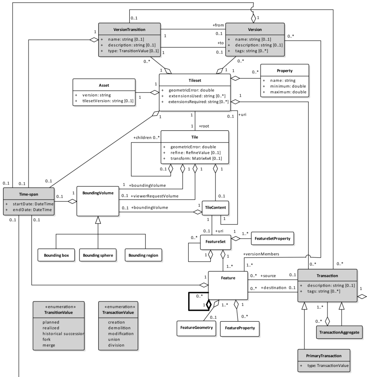
Figure 6. Logic4DCity :_UML logical model for time-evolving 3D city models on the web based on extending 3D Tiles. A logical model of 3D Tiles, Logic3DCity , is proposed in white and the temporal extension is represented in gray. The recursive composition association of Feature (thick line) is a conceptual representation of the batch_table_hierarchy extension of 3D Tiles.
