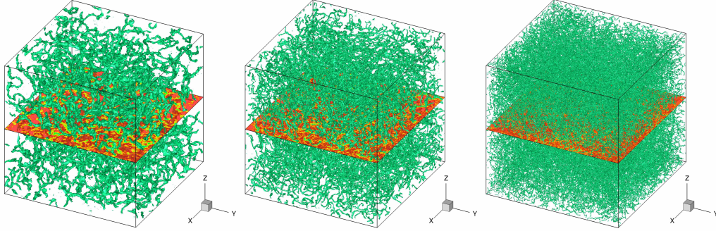
Figure 11: ABC-QT. Instantaneous fields computed with the real-time GP solver, starting from the initial condition presented in Fig. 9. Vortex lines (iso-surfaces of low \rho ) of the wave function at final time T_f . From left to right: grid resolutions N_x = 128, 256, 512 (corresponding to runs ABC_a, ABC_b and ABC_c in Table 7).
