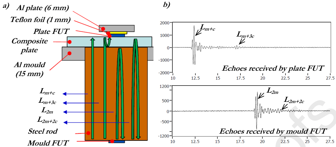
Figure 2. Schemes of a) the FUT assembly and b) the different echoes produced by the FUT for composites curing monitoring.
