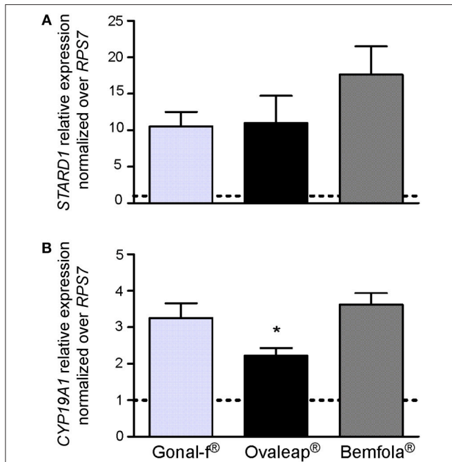
FIGURE 4 | STARD1 and CYP19A1 gene expression analysis. The expression of STARD1 (A) and CYP19A1 (B) gene was evaluated in hGLC stimulated for 12 h with the EC 50 of Gonadotropin Releasing Hormone (Gonal-f ® ) or biosimilars (12 ng/ml Gonadotropin Releasing Hormone (Gonal-f ® ) and Ovaleap ® , 24 ng/ml Bemfola ® ) by real-time PCR. Each value was normalized over the RPS7 gene expression (means ± SEM; n = 4). Unstimulated cells served as control and are indicated as a dotted line. (*= significant vs. Bemfola ® , Kruskal Wallis test; p < 0.05).
