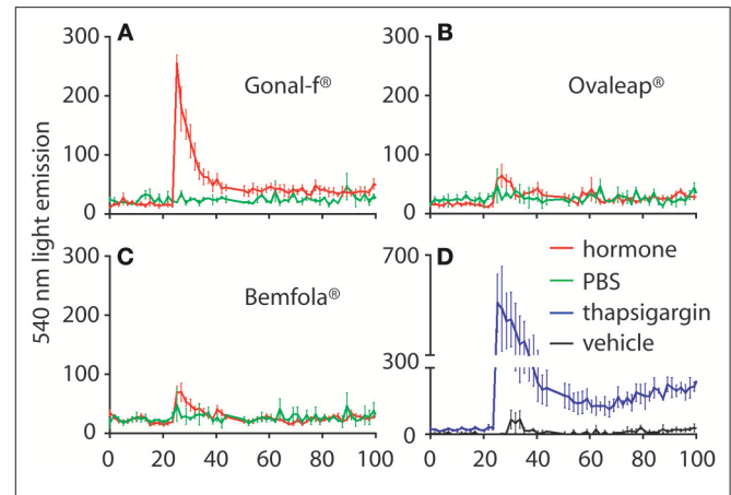
FIGURE 5 | Calcium response kinetics in transfected HEK293 cells treated with Gonadotropin Releasing Hormone (Gonal-f ® ) or biosimilars. Cells were transiently co-transfected with FSHR and aequorin sensors, then stimulated in duplicates with a fixed dose (4 × 10 3 ng/ml) of (A) Gonadotropin Releasing Hormone (Gonal-f ® ), (B) Ovaleap ® , (C) Bemfola ® . (D) Thapsigargin, PBS and hormone diluent were used as positive and negative controls, respectively. BRET signal was measured for 100 s. Data are represented as means ± SEM (n = 3). Area under the curve (AUC) values were calculated and differences were considered for p < 0.05 (Kruskal Wallis test).
