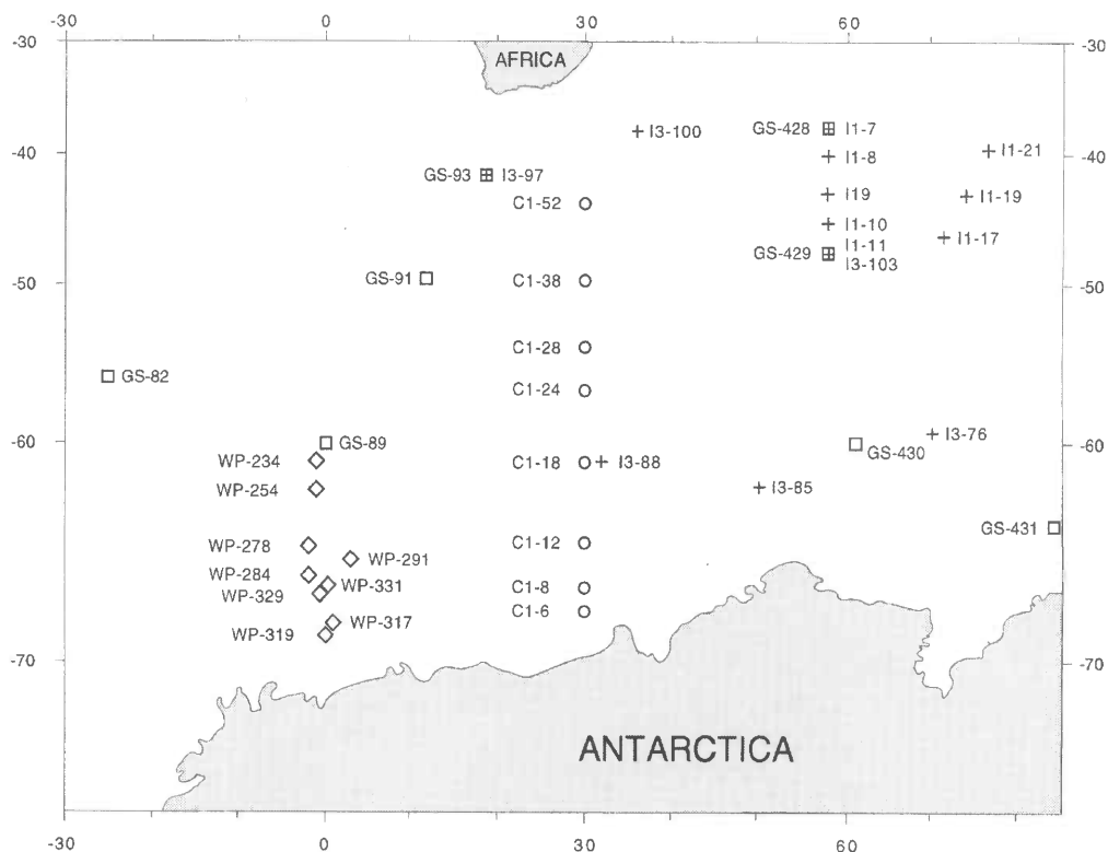
Figure 2 Stations occupied to collect samples for ^{14}\text{C} during CIVA1 (C1) as well as adjacent ^{14}\text{C} stations from GEO-SECS (GS), WWSWP (WP), INDIGO (I1 and I3)
